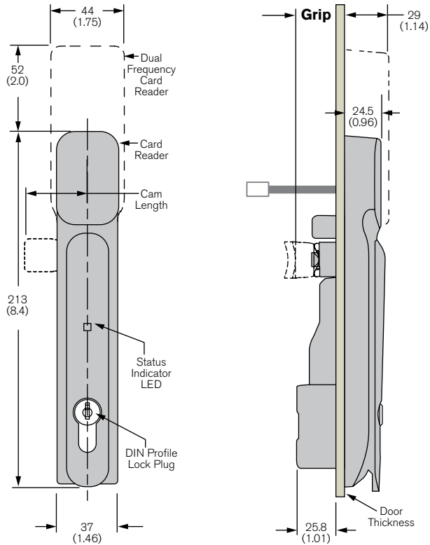
Electronic Swinghandle Dimensions:
